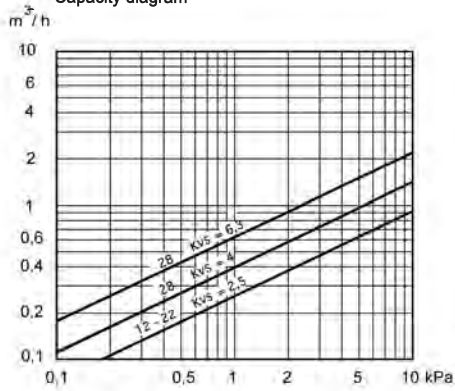
Capacity diagram
