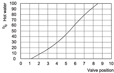
Mixing characteristic
